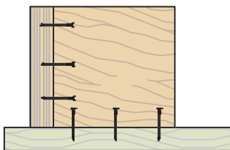
(a) Block skew nailed to beam and to support with 3/75 mm skew nails to each member.
